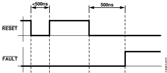
Figure 23. \overline{\text{RESET}} Timing
