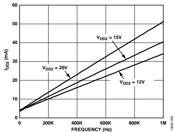
Figure 9. Typical I_{DD2} Current vs. Frequency, Duty = 50%, 2 nF Load, V_{SS2} = 0 V
