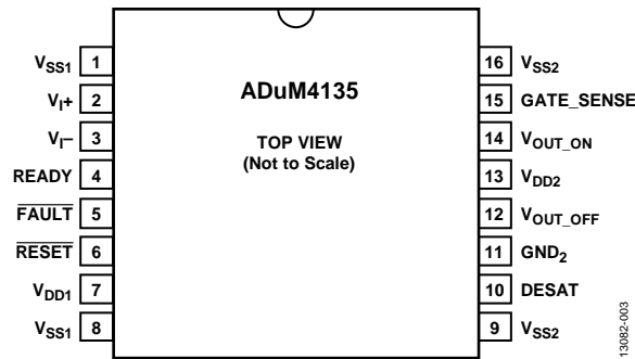
Figure 3. Pin Configuration
