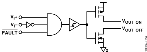
Figure 24. V_{I+} and V_{I-} Block Diagram
