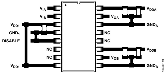
Figure 19. Recommended PCB Layout
