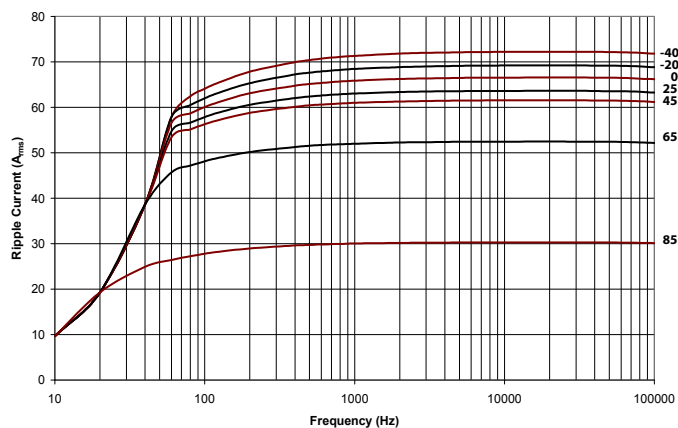
947D641K901AHGSN Rated Ripple Current, Still Air, 7kh Life
