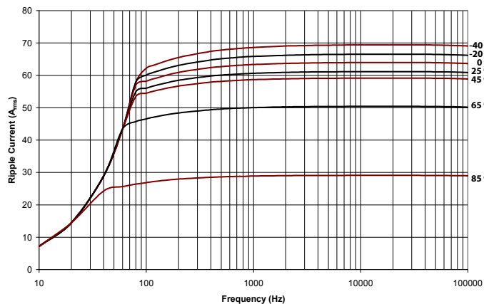
947D481K112ALGSN Rated Ripple Current, Still Air, 7kh Life
