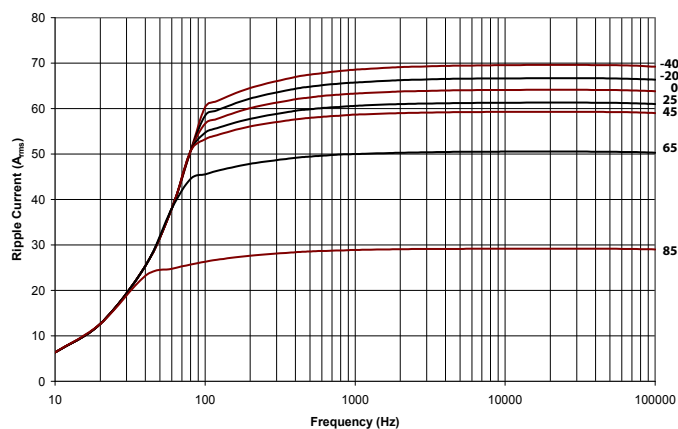
947D421K112AHGSN Rated Ripple Current, Still Air, 7kh Life
