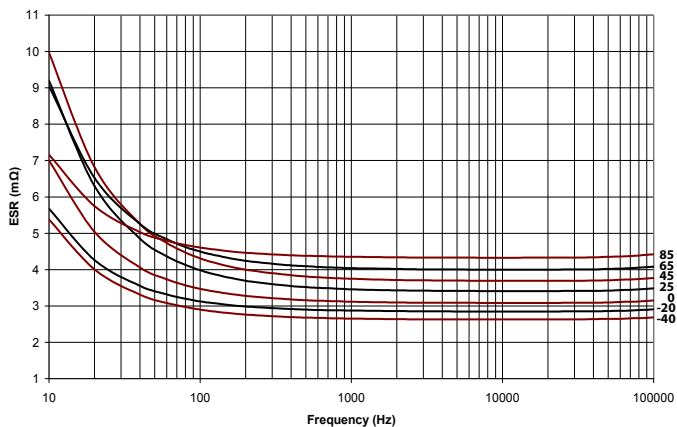
947D481K112ALGSN ESR vs Frequency and Temperature
