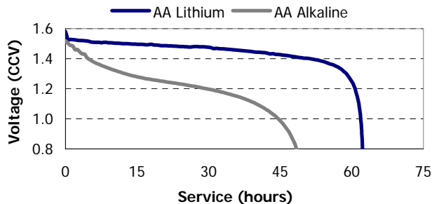
Low Drain Performance 50mA Continuous (21°C)
