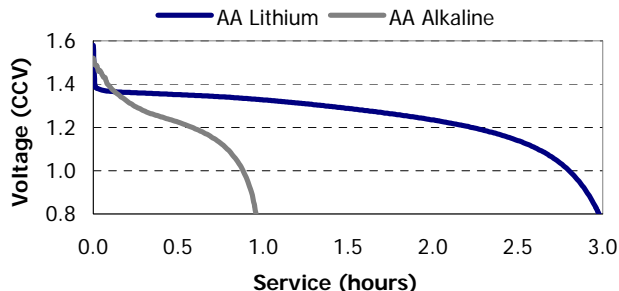
High Drain Performance 1000mA Continuous (21°C)
