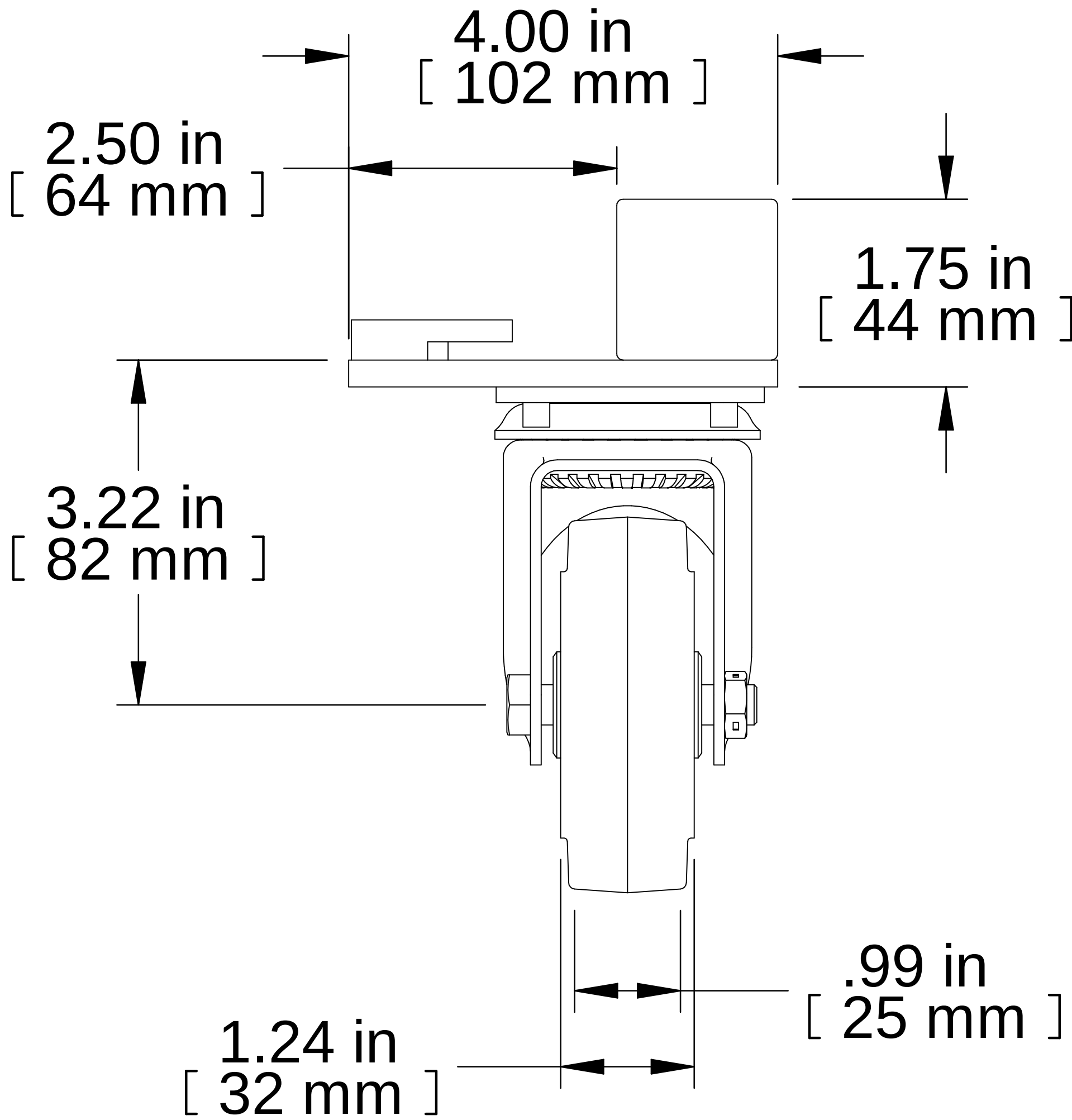
FRONT VIEW
