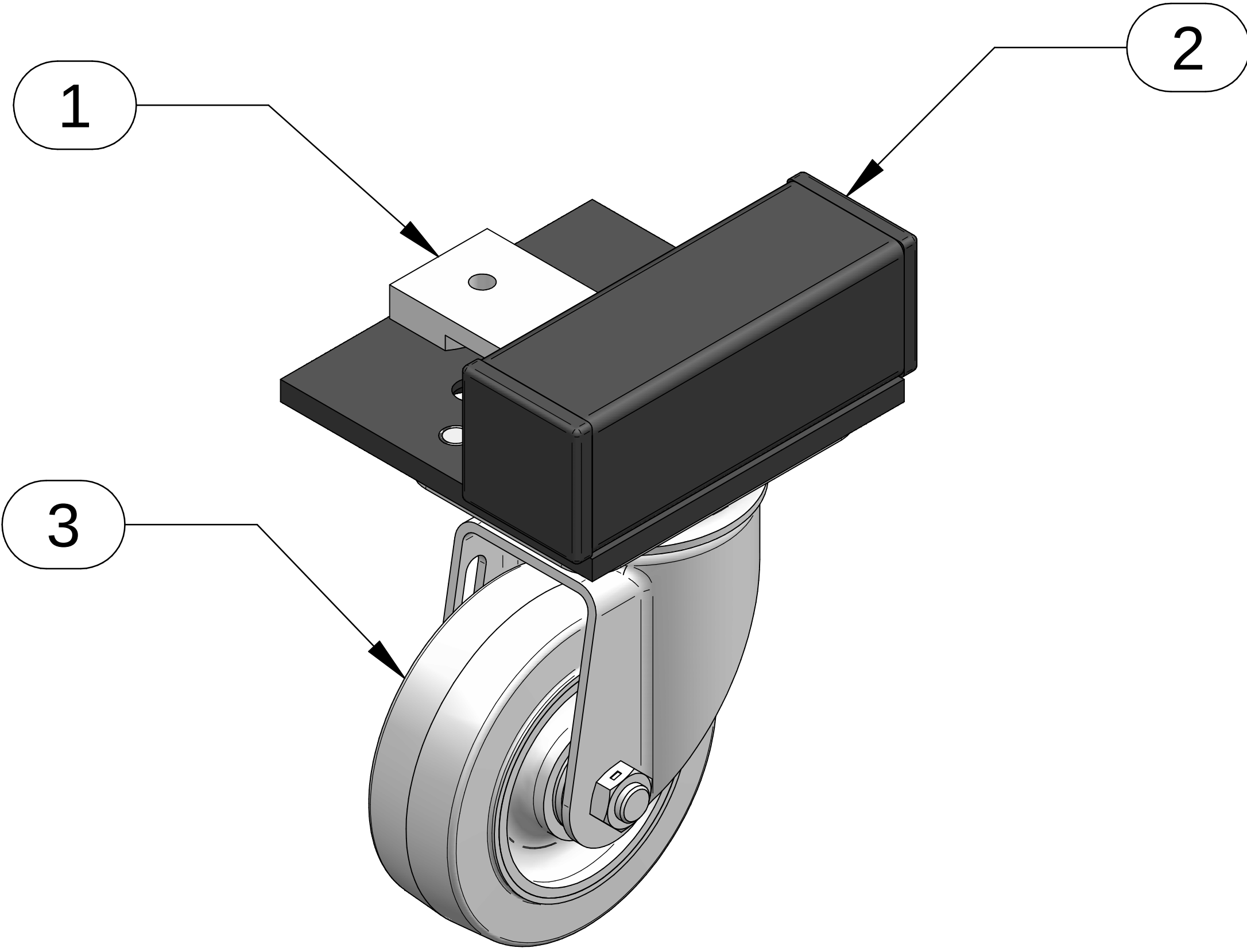
ISOMETRIC
