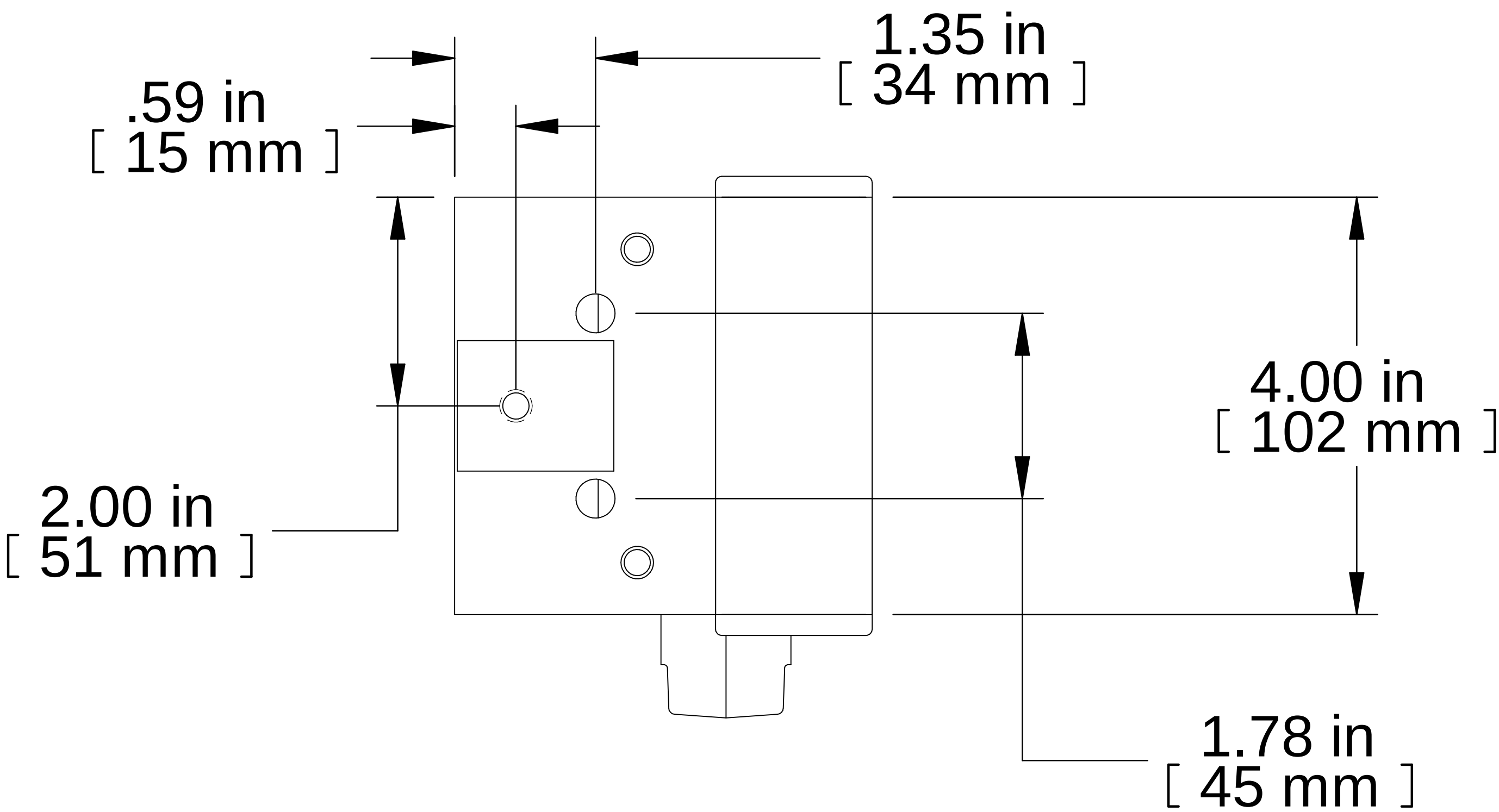
TOP VIEW
