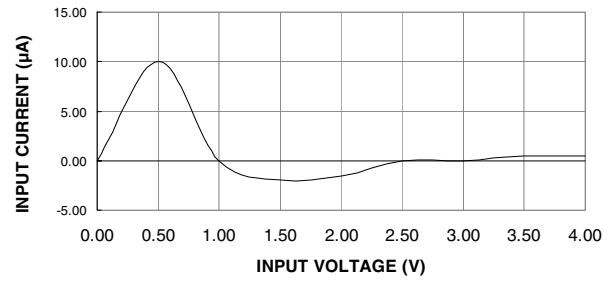
ATF22LV10C INPUT CURRENT VS. INPUT VOLTAGE ( V_{CC} = 3.3V , T_A = 25^\circ C )
