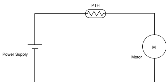
(1) DC Motor Protection Circuit
