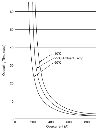
PTGL09AR470M6B52B0
