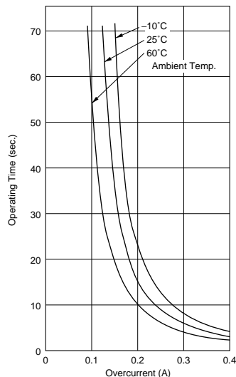
PTGL07AR750M7B52B0
