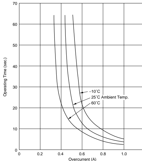
PTGL07AR4R6H2B51B0
