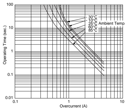
PTGL07AS2R7K2B51B0
