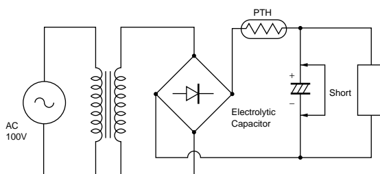
(4) Short - Circuit Test of Electrolytic Capacitor
