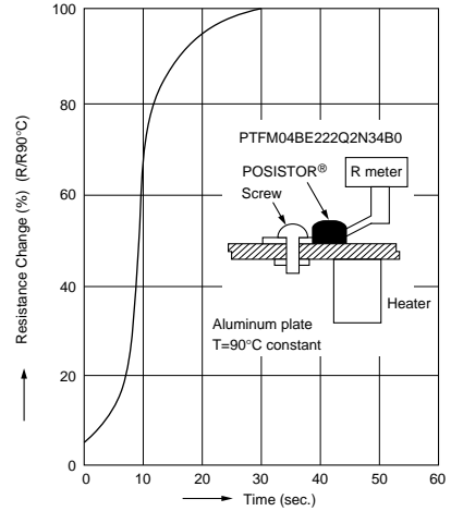
Relation between resistance change and time after POSISTOR® PTFM04BE222Q2N34B0 is installed on the part heated at a constant temperature of 90°C (3mm thick alumin sheet) is shown in the figure below.
