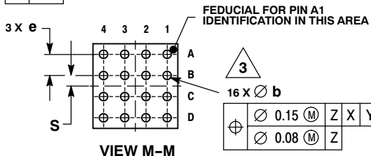
VIEW M-M
