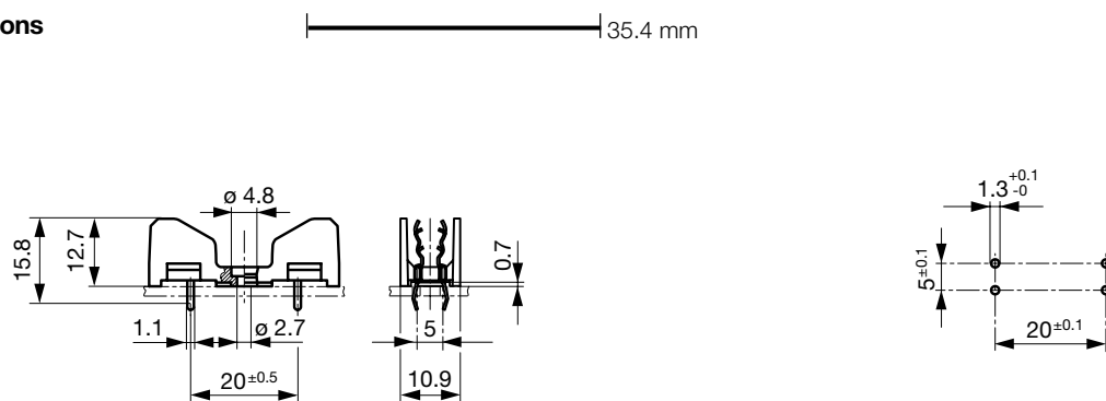
Drilling diagram
