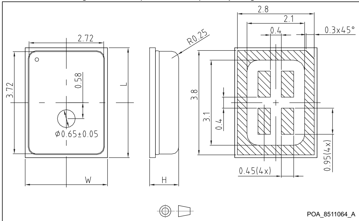
Figure 5. HCLGA (3 x 4 x 1.06 mm) 4-lead package outline
