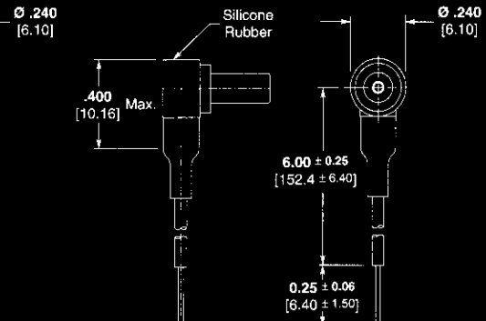
Plug (Right-Angle) Part Number 448661-1
