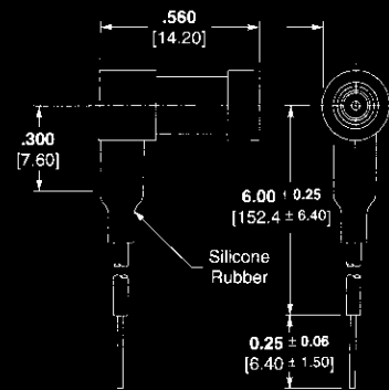
Receptacle (Right-Angle) Part Number 448659-1
