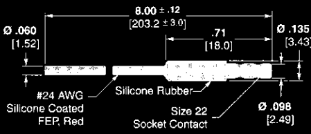
Plug Part Number 443957-1
