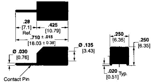
Receptacle, Surface Mount Part Number 1218055-1 Glass Filled Epoxy, Black Part Number 1218055-2 PPS Thermoplastic Polymer, Brown
