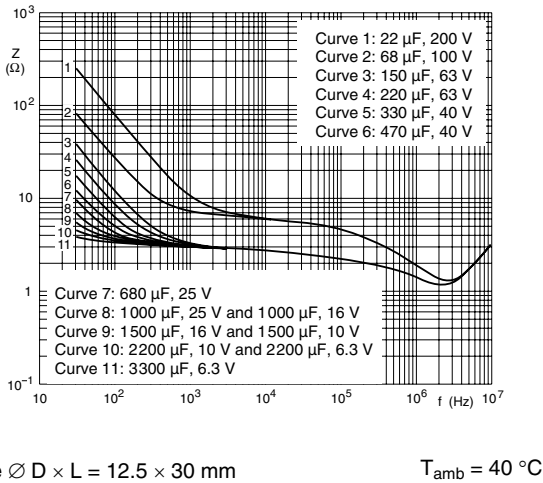
Fig.15 Typical impedance as a function of frequency
