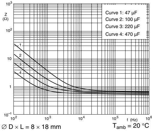
Fig.13 Typical impedance as a function of frequency
