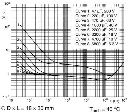
Fig.17 Typical impedance as a function of frequency
