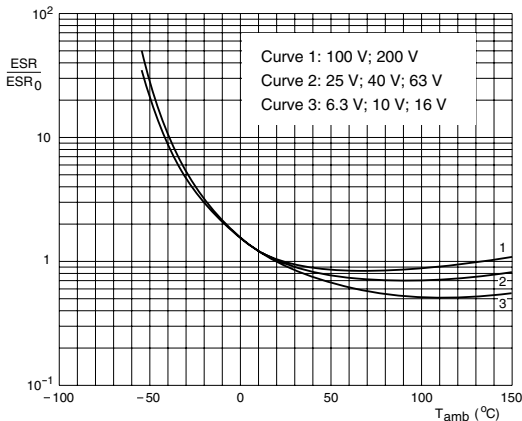
Case \varnothing D \times L = 6.5 \times 18 to 15 \times 30 mm ESR_0 = typical at 20 °C; 100 Hz
