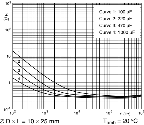
Fig.14 Typical impedance as a function of frequency
