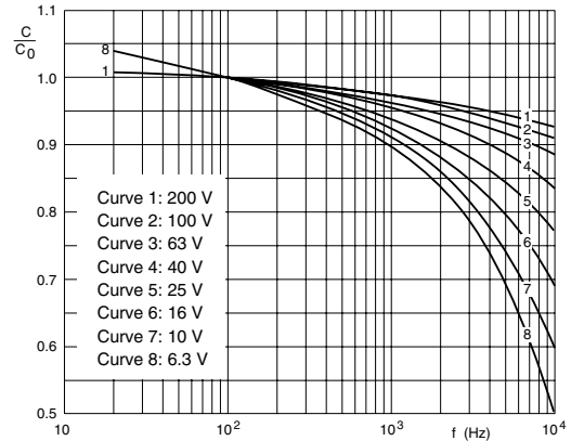
Case \varnothing D \times L = 10 \times 30 to 21 \times 38 mm C_0 = capacitance at 20 °C; 100 Hz
