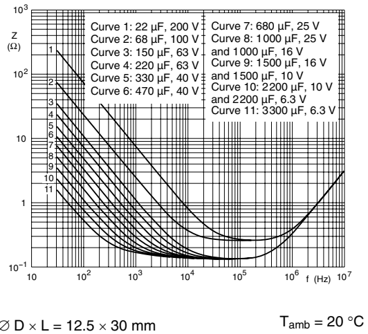
Fig.16 Typical impedance as a function of frequency
