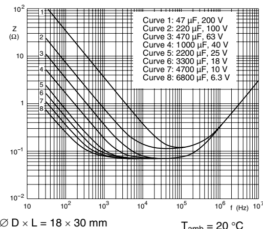
Fig.18 Typical impedance as a function of frequency
