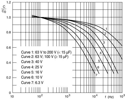
Case \varnothing D \times L = 6.5 \times 18 to 10 \times 25 mm C_0 = capacitance at 20 °C; 100 Hz
