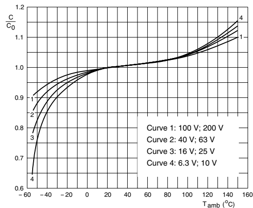
Case \varnothing D \times L = 10 \times 30 to 21 \times 38 mm C_0 = capacitance at 20 \text{ }^\circ\text{C} , 100 Hz
